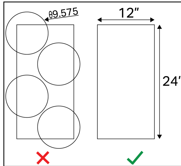
Figure 35: Custom plastic parts must fit within a single 12" x 24" sheet of plastic.
