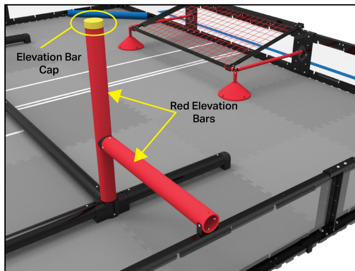
Figure 11: An Elevation Bar and Elevation Bar Cap.
